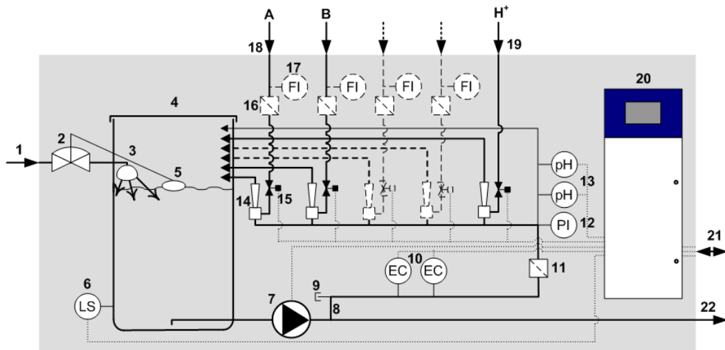
NutriFit fertiliser dosing unit diagram
