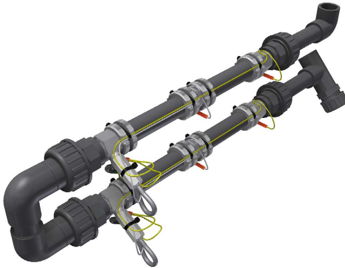
Measuring tube with 2 EC sensors
